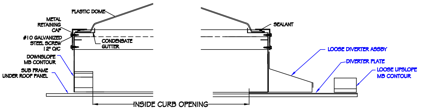
CURBS AND SKYLIGHTS SHIPPED LOOSE FOR FIELD ASSEMBLY
