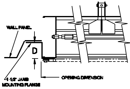
TYPICAL JAMB
