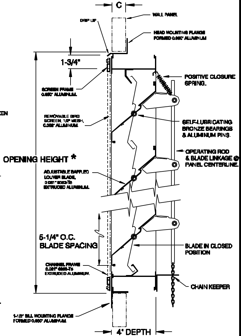
VERTICAL SECTION
