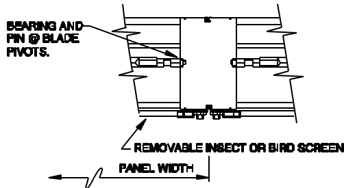
TYPICAL MULLION
