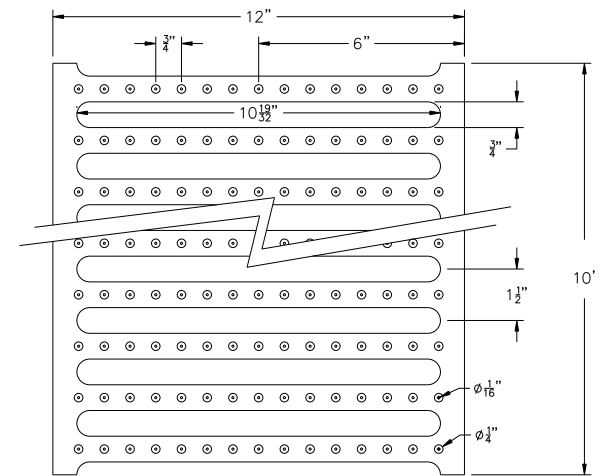
SIDEVIEW C
